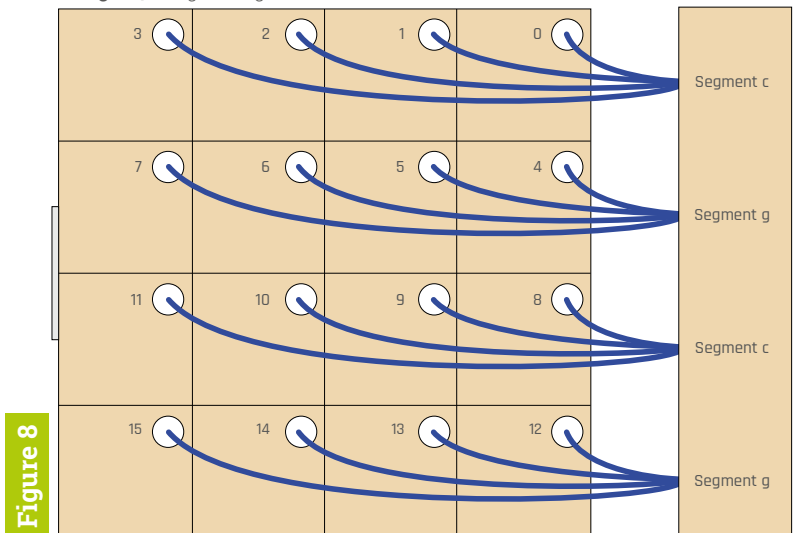
▲ Figure 8 The blue segment c & g wires
