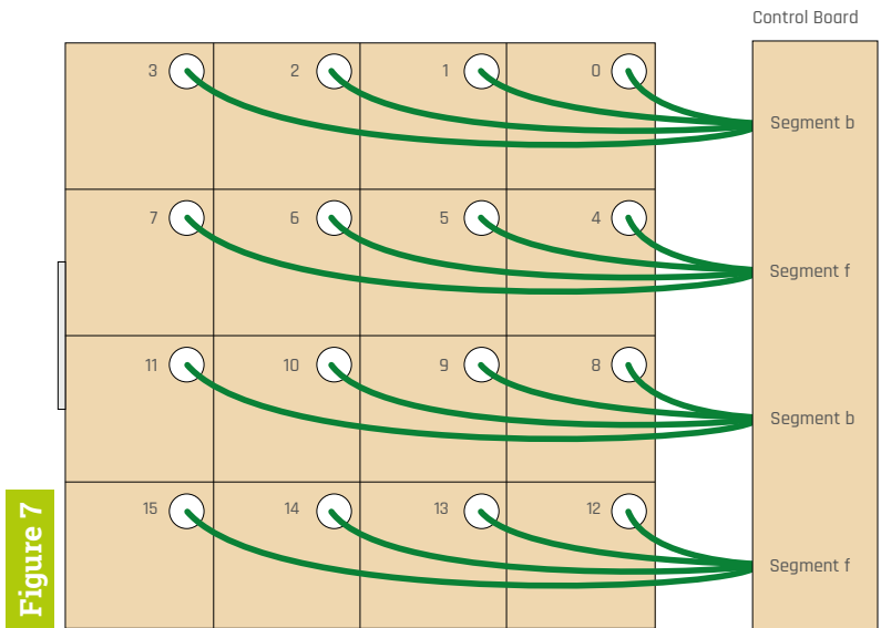
▲ Figure 7 The green segment b & f wires
