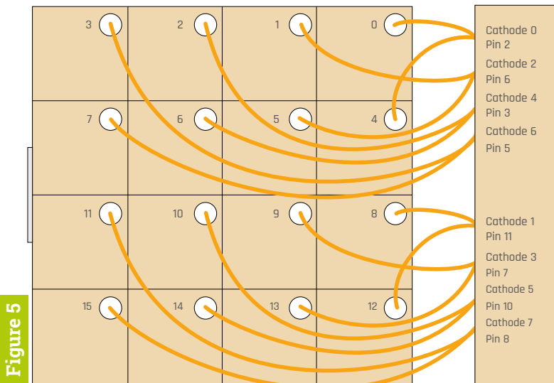
▲ Figure 5 The orange cathode wires
