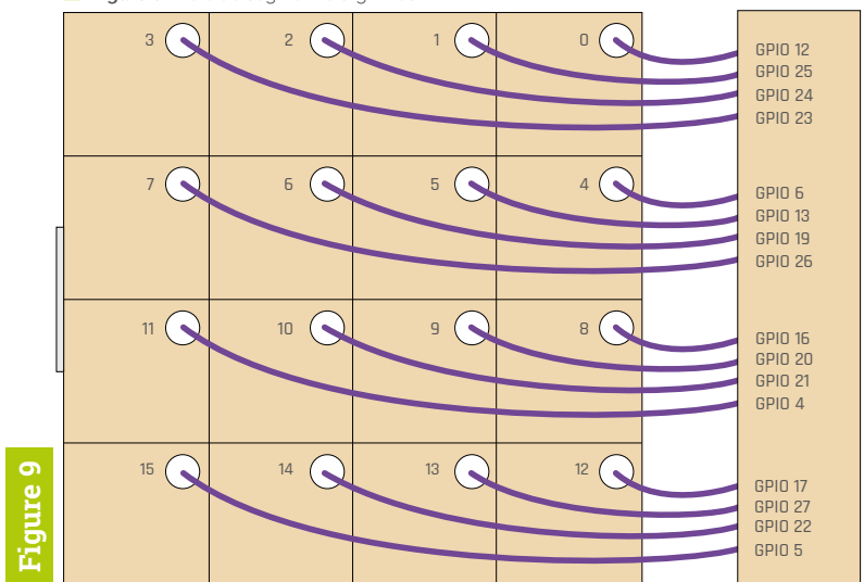
▲ Figure 9 The violet switch wires
