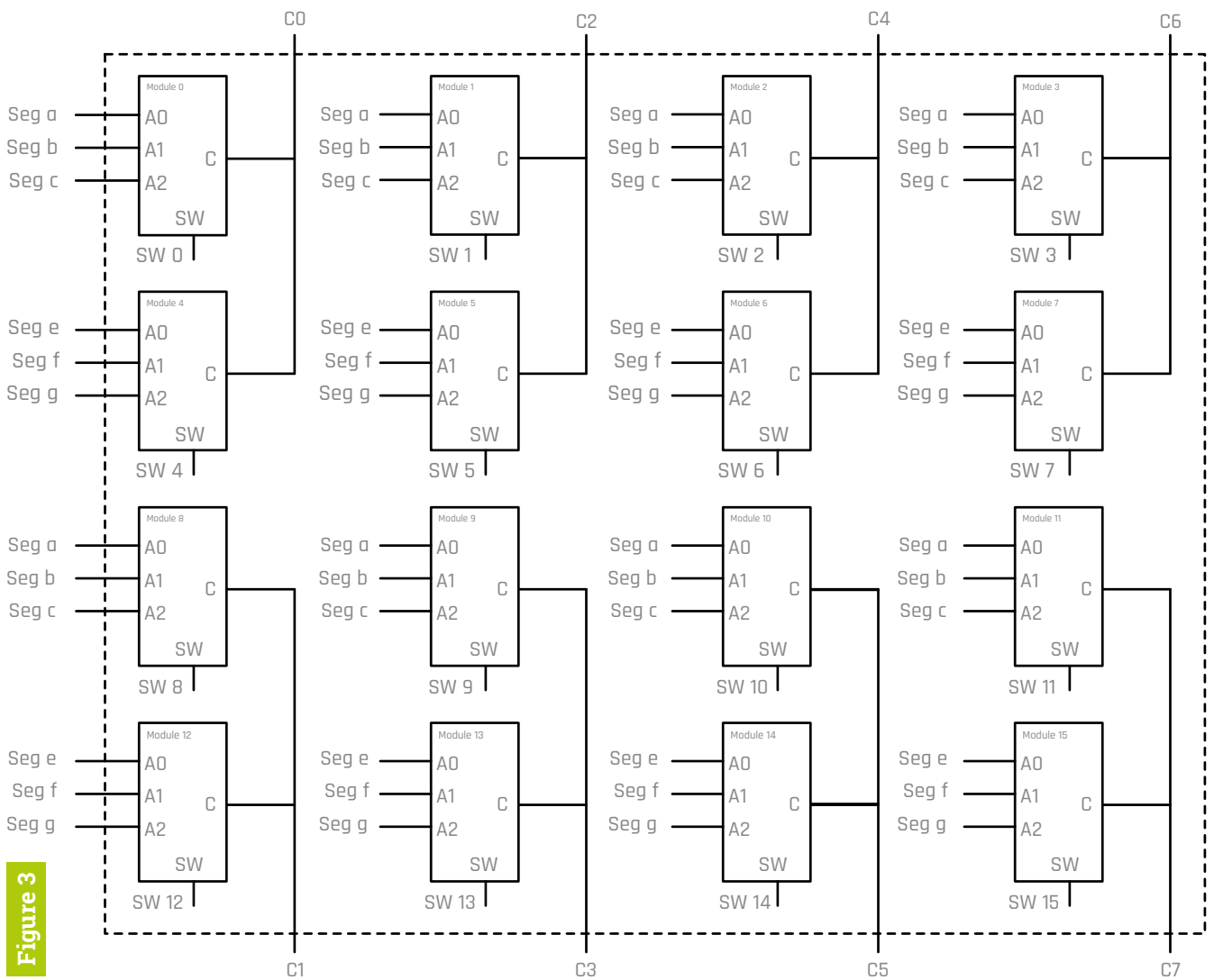
▼ Figure 3 The schematic of the matrix made from LED boards
