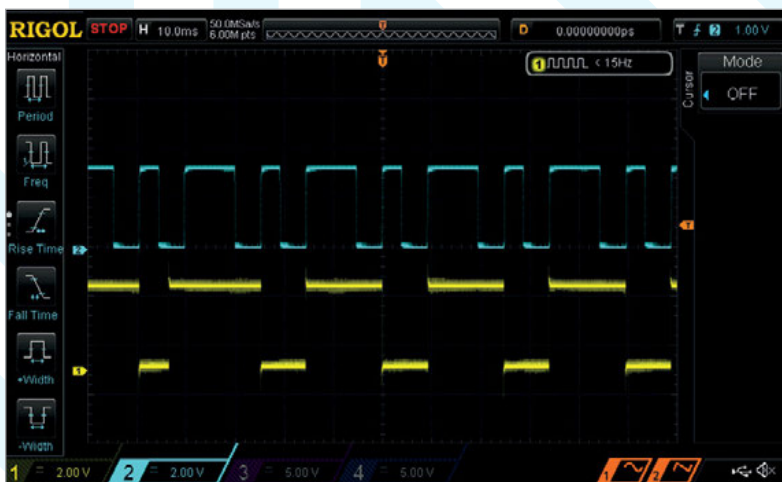
Figure 3 Oscilloscope trace showing the input pulse (top trace) and the GPIO output feedback (bottom trace)
